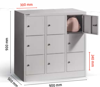
PARAPET 3/9 NEW
